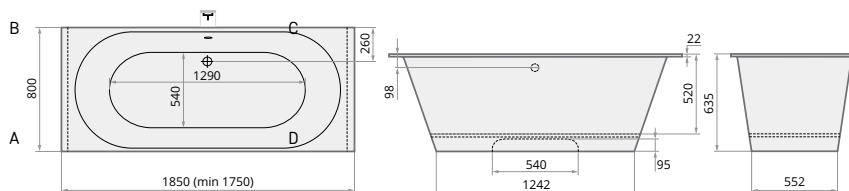
VARIO XL 1850 × 800 mm 1750-1850 × 800 mm h = 635 mm Tilpums: 240 l Svars: 135 kg
