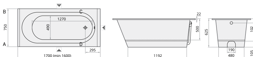
VARIO L 1700 × 750 mm 1600-1700 × 750 mm h = 625 mm Tilpums: 220 l Svars: 107 kg
