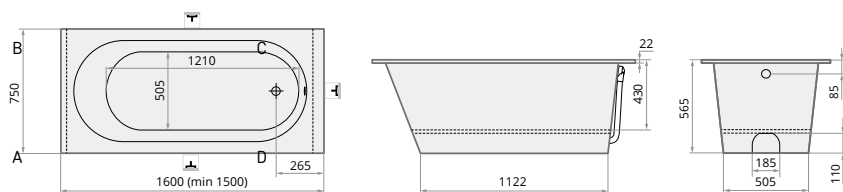
VARIO M 1600 × 750 mm 1500-1600 × 750 mm h = 565 mm Tilpums: 200 l Svars: 100 kg
