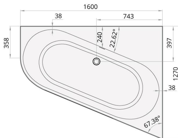
DECO CORNER A, 1600x1270
