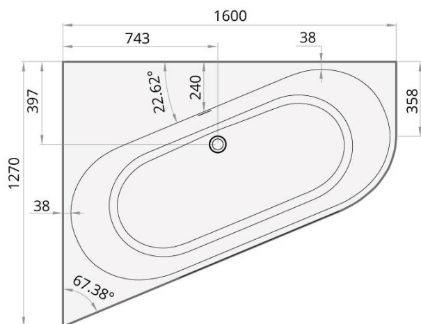
DECO CORNER D, 1600x1270
